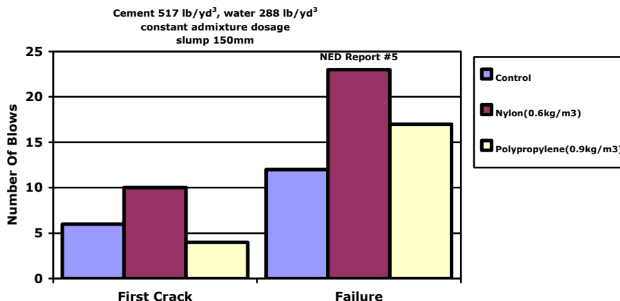
Figure 2-Impact Resistance
